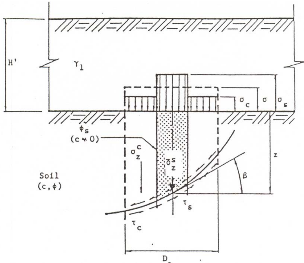
Figure 5-22. Notation used in average stress method stability analysis.
