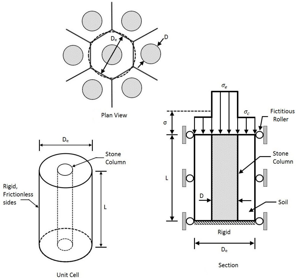
Figure 5-17. Unit cell idealization.
